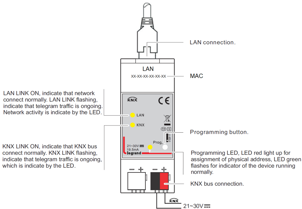
Fig. 3.2.1 Connection diagram
